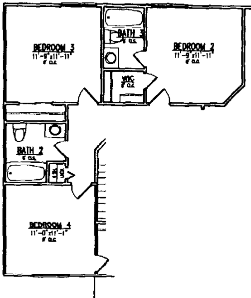
OPT. BATH 3 W/ BEDROOM 2 RMS 02400
