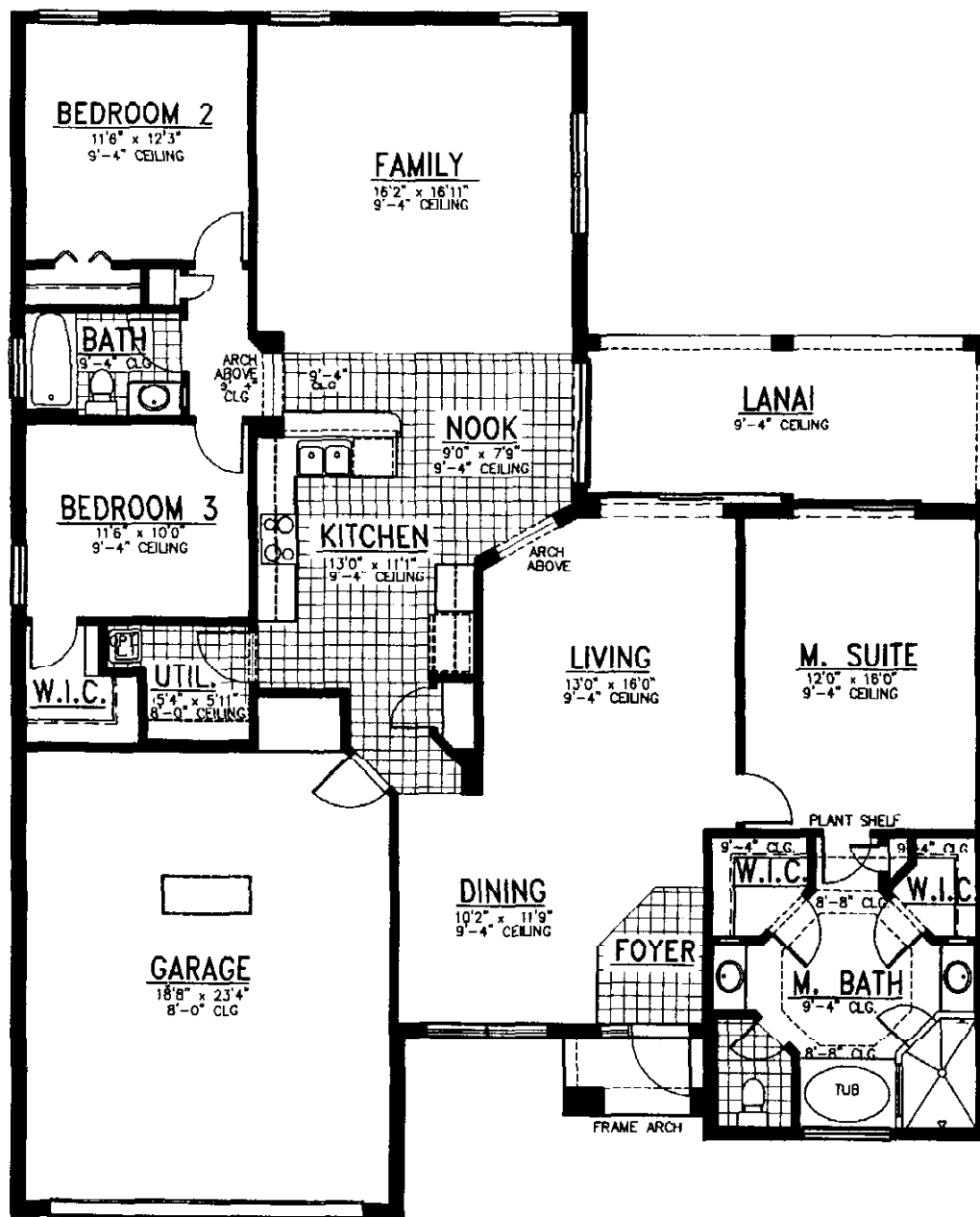
FLOOR PLAN
